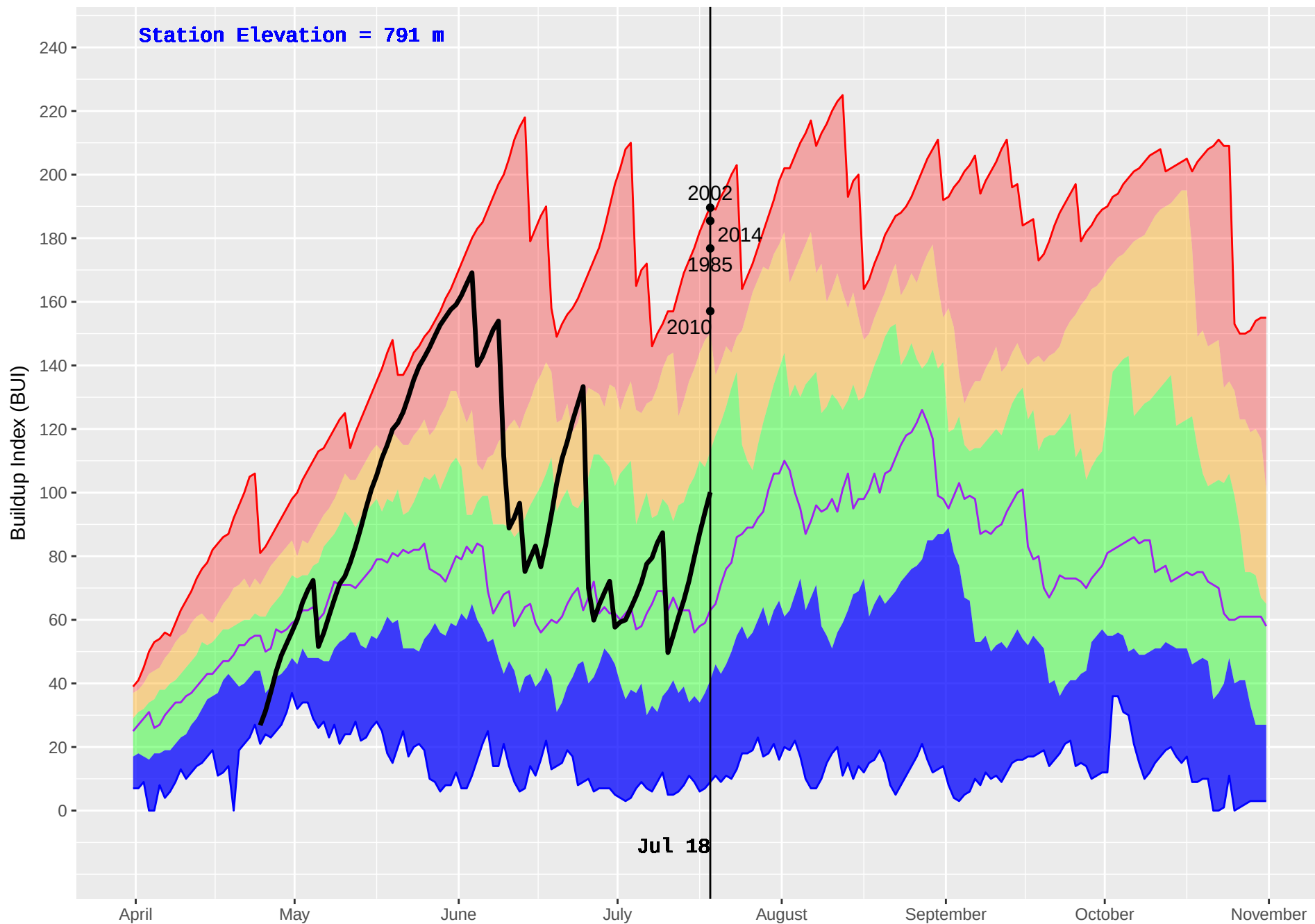
ALEXIS CREEK (209) : Historical (1980–2016) and Current (2018) Daily Buildup Index (BUI)
