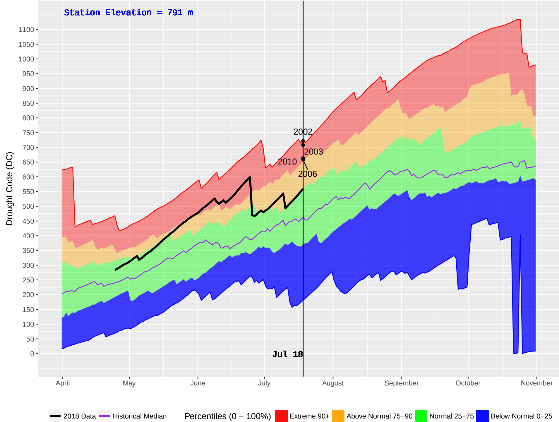
ALEXIS CREEK (209) : Historical (1980–2016) and Current (2018) Daily Drought Code (DC)
