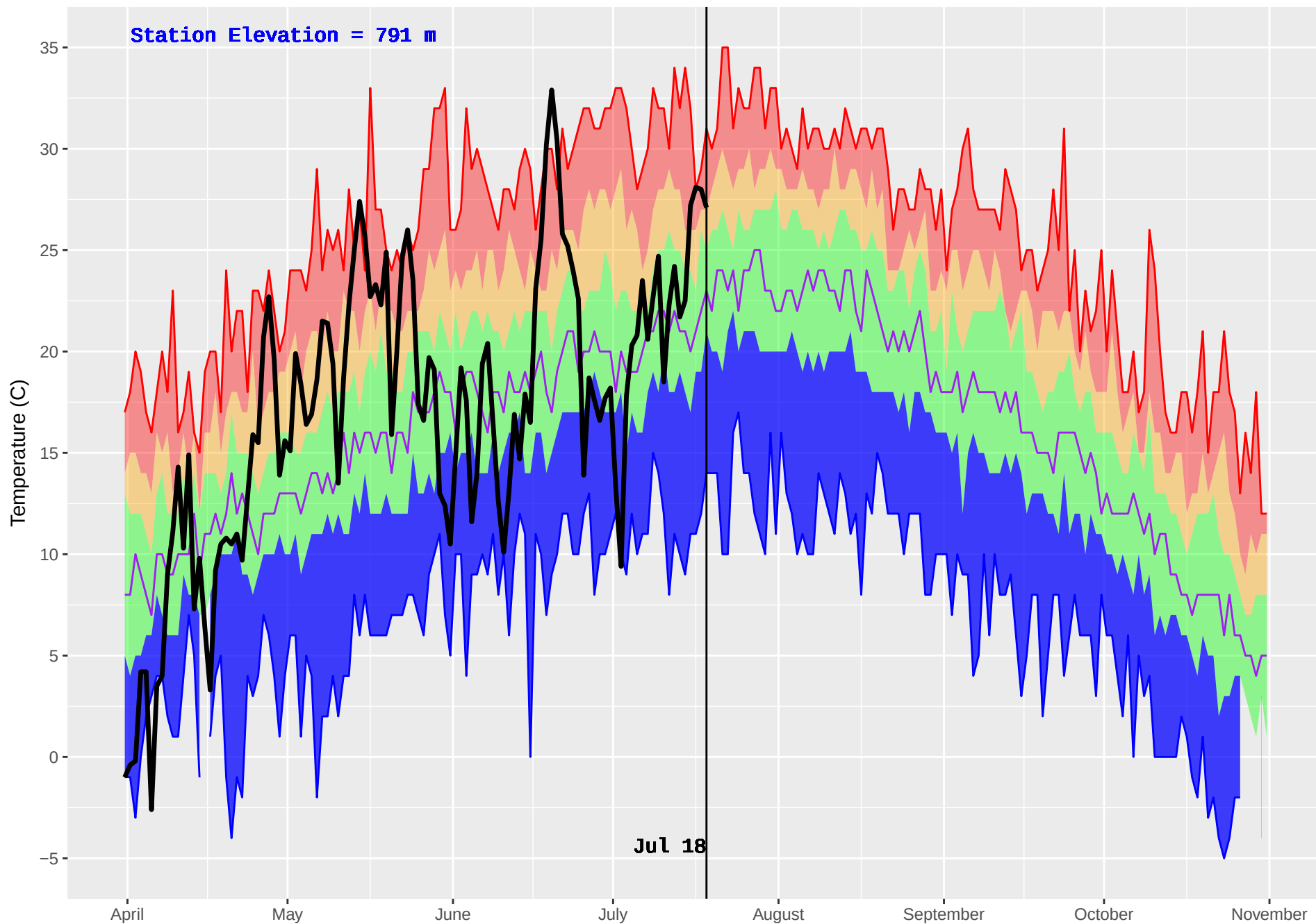
ALEXIS CREEK (209) : Historical (1980–2016) and Current (2018) Daily Temperature
